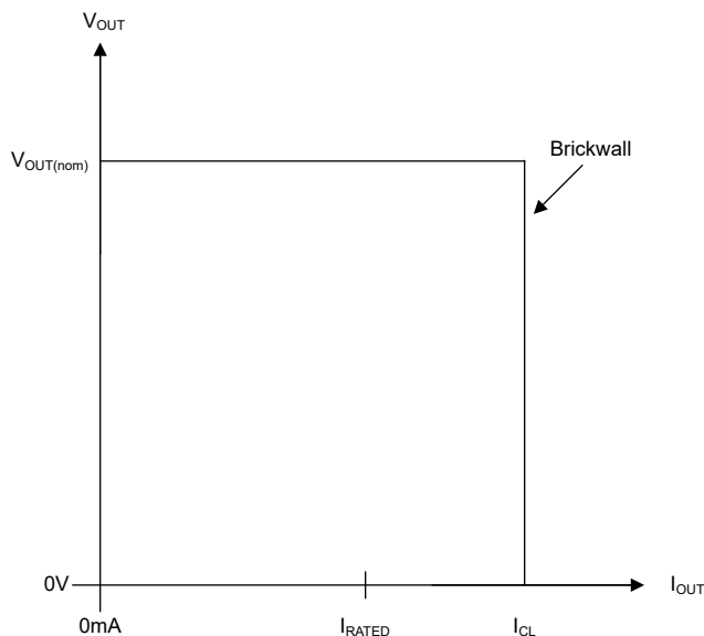
Figure 7-1. Current Limit
