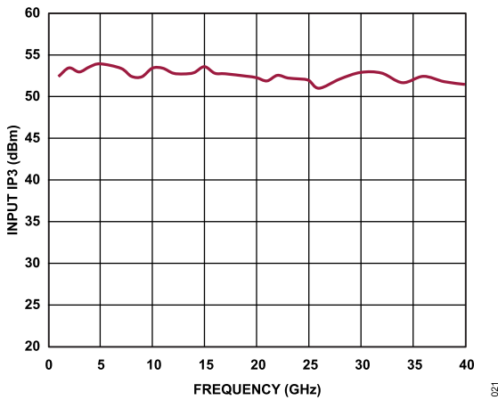
Figure 21. Input IP3 vs. Frequency
