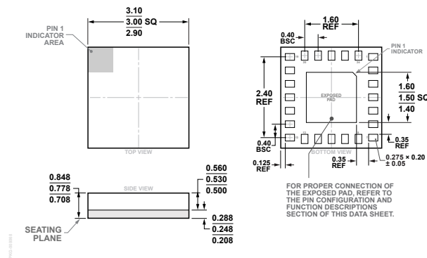
Figure 28. 24-Terminal Land Grid Array [LGA] (CC-24-14) Dimensions shown in millimeters
