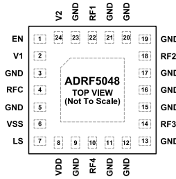
Figure 4. Pin Configuration
