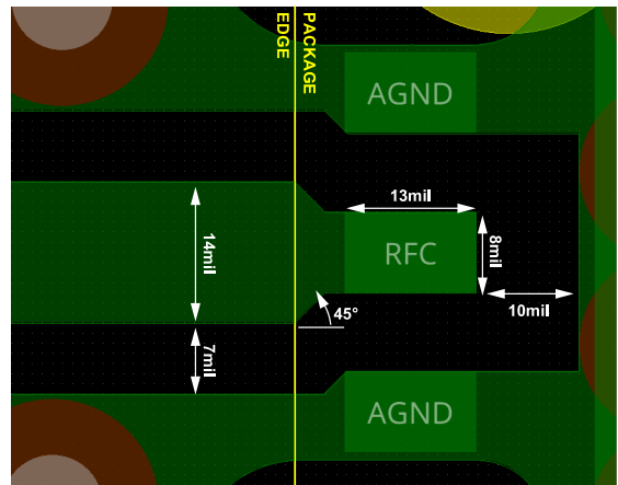
Figure 27. Recommended RFx Pin Transitions
