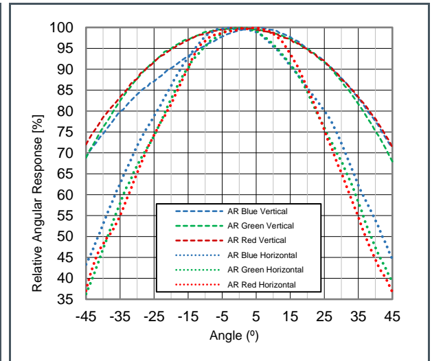
Figure 24: 4LS RGB Relative Angular Response (1)(2)
