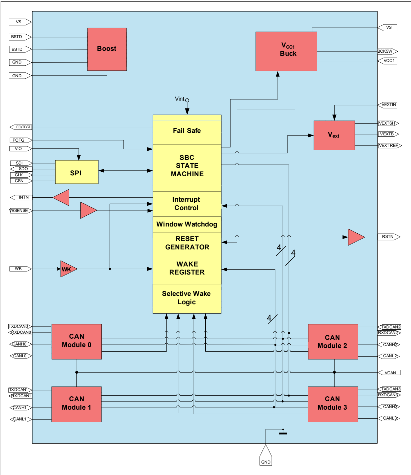
Figure 1 Block Diagram
