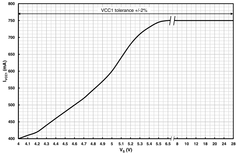
Figure 18 Maximum DCDC Buck current capability versus V_S
