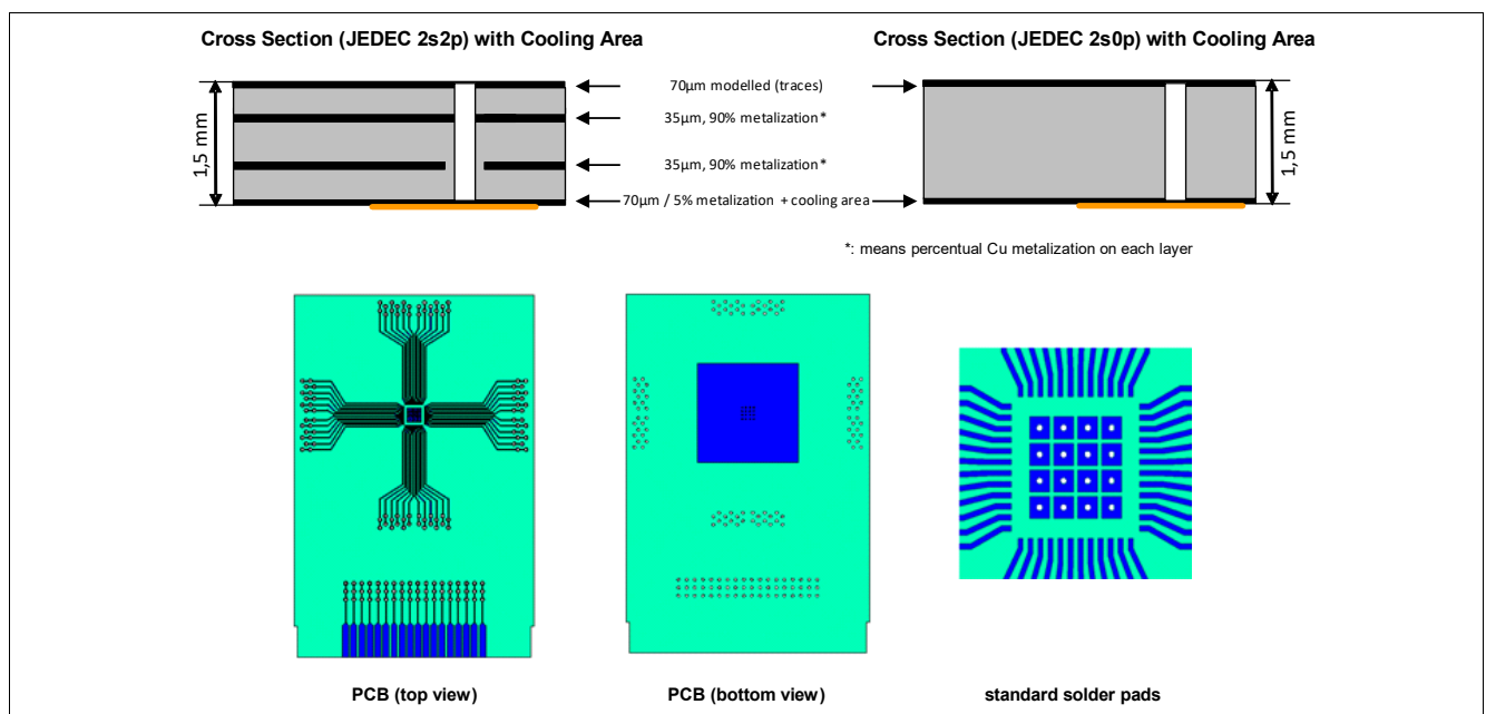
Figure 55 Board Setup
