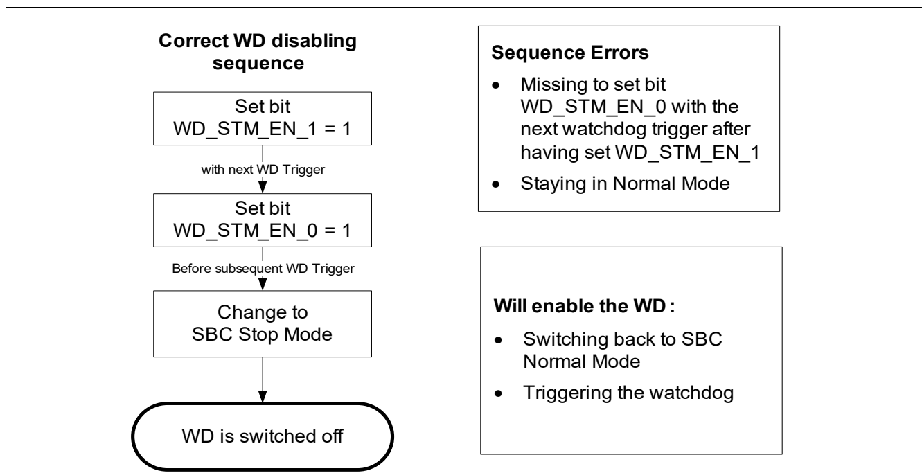
Figure 40 Watchdog Disabling Sequence
